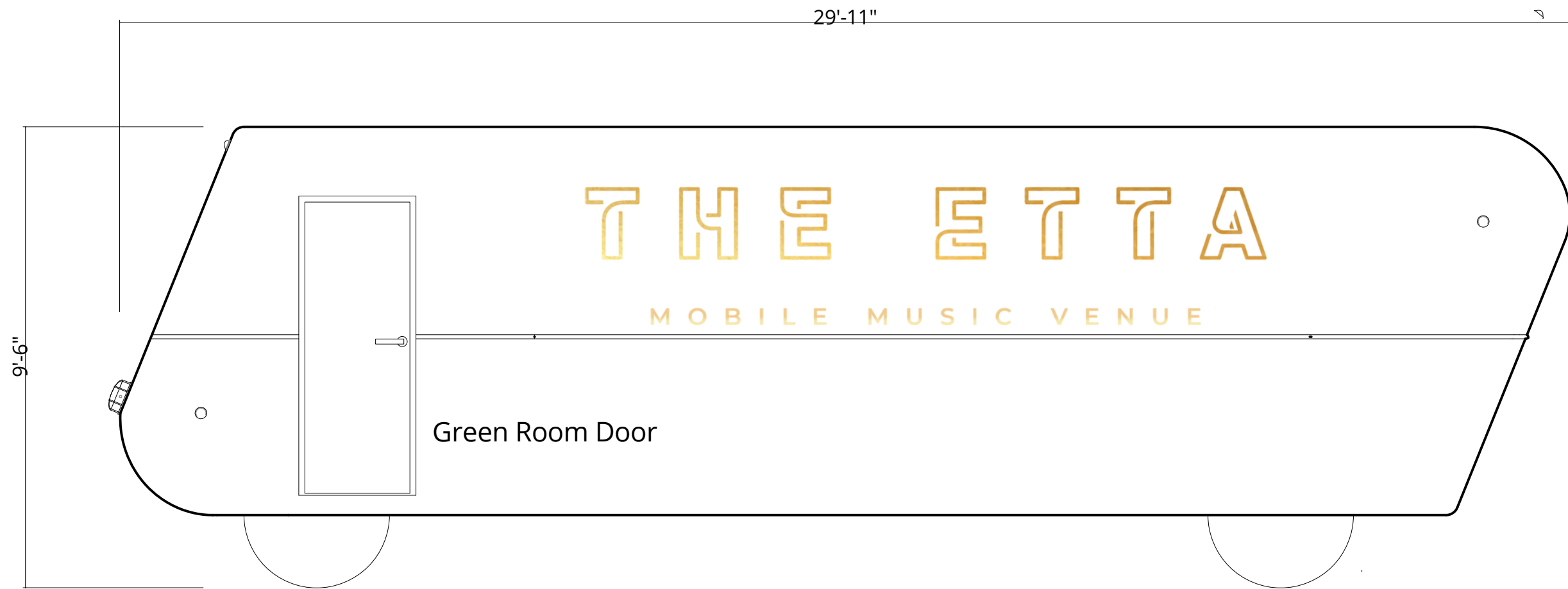
The Etta Elevation Green Room Access
